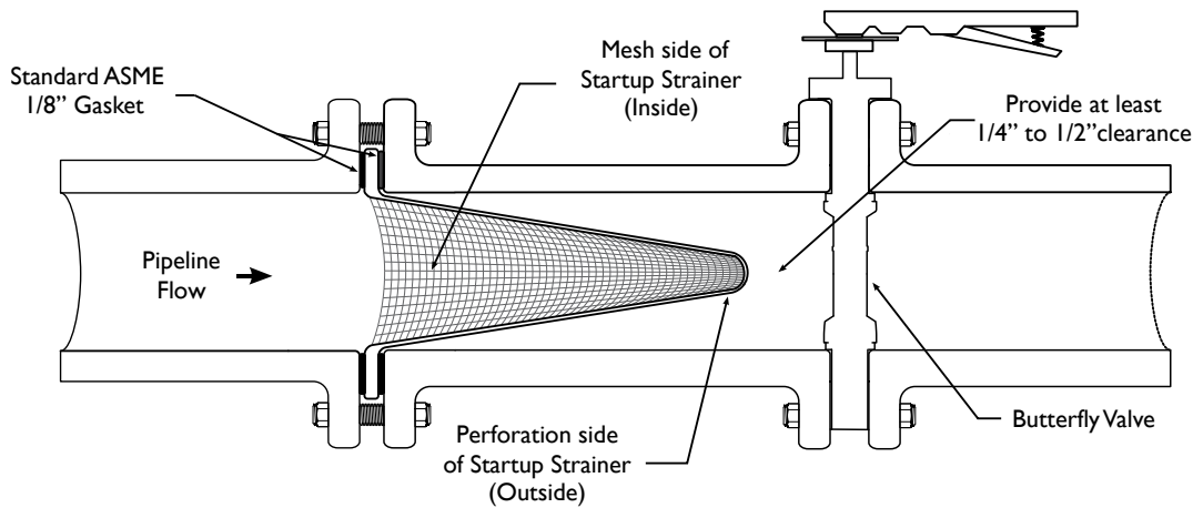
Figure 3: Simplified Drawing of an Installed Startup Strainer
